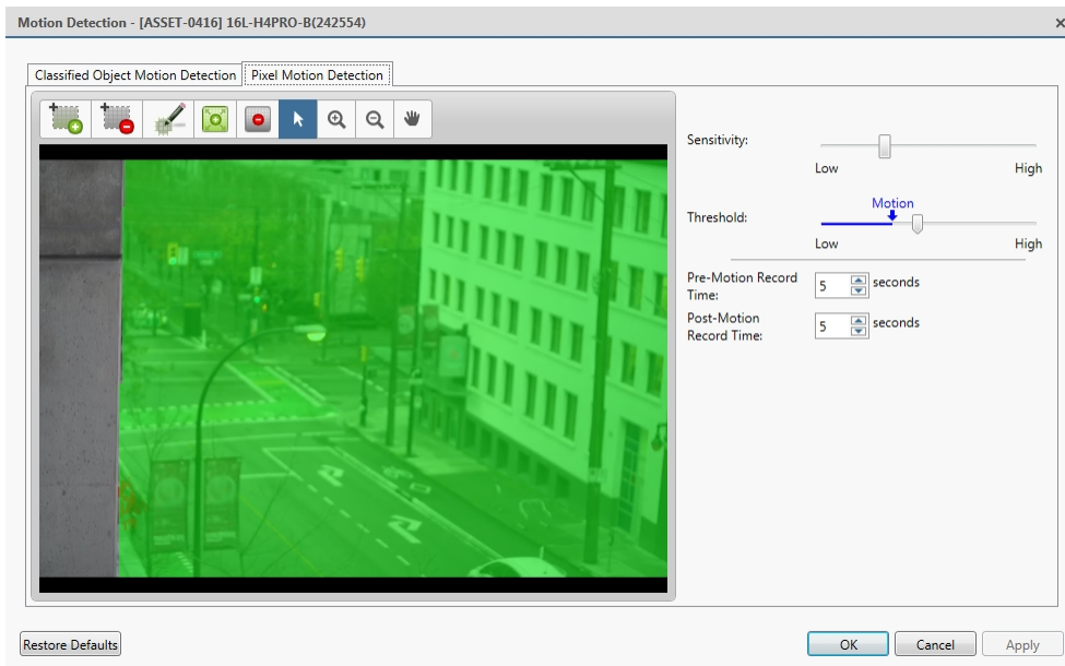
Figure 8: The Motion Detection dialog box: the Pixel Motion Detection tab
